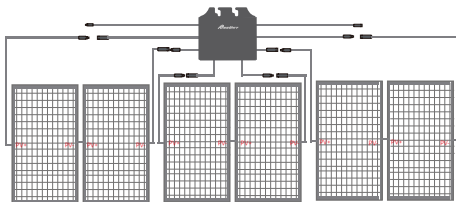
AW-PVRS-A6/B6/C6 1:6 Connection Diagram
