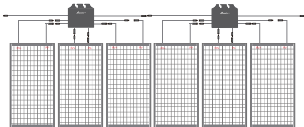
AW-PVRS-A3/B3/C3 1:3 String Parallel Connection Diagram
