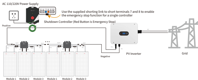
AW-PVRS-A3/B3/C3 1:3 Controller Connection Diagram
