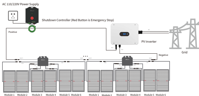
AW-PVRS-A6/B6/C6 1:6 Controller Connection Diagram
