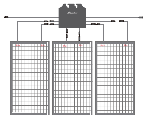
AW-PVRS-A3/B3/C3 1:3 Connection Diagram
